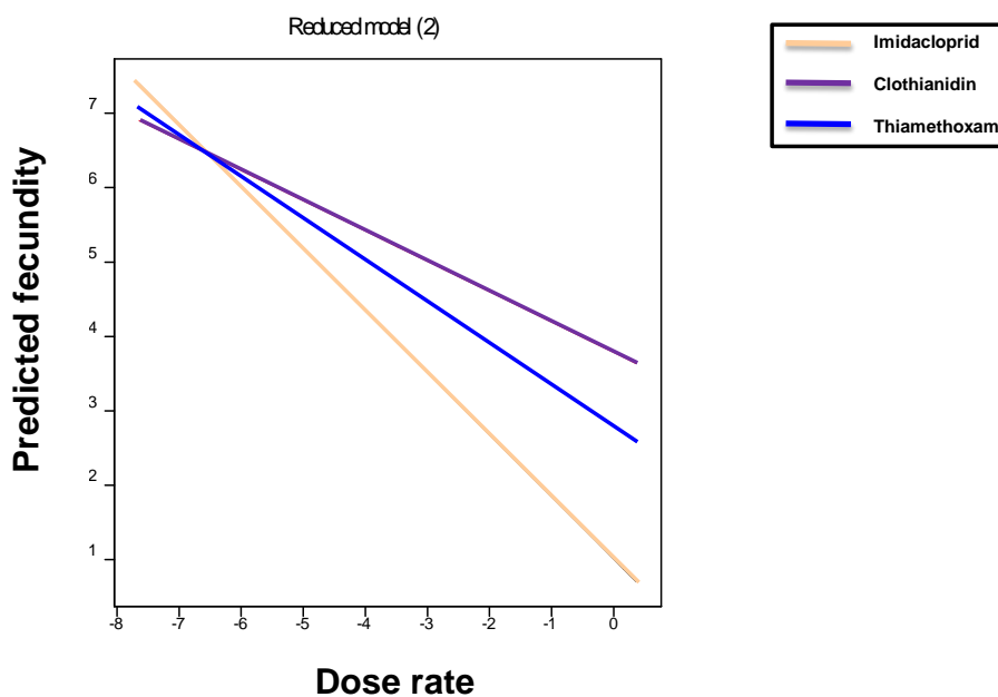
Figure 14. Fecundity (at 3-5 days) versus dose rate of the Nic-S, Nic-R and Nic-R+ Myzus persicae clones (pooled) exposed to actual doses of imidacloprid, clothianidin and thiamethoxam seed-treated oilseed rape plants. X axis: \text{Log}_2(\text{Dose}+0.005) ; Y axis: \text{Sqrt}(\text{Number of nymphs days 3-5}) .
