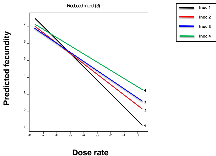
Figure 15. Fecundity at each inoculation versus dose rate of the Nic-S, Nic-R and Nic-R+ Myzus persicae clones exposed to imidacloprid, clothianidin and thiamethoxam (pooled) seed-treated oilseed rape plants. X axis: \text{Log}_2(\text{Dose}+0.005) ; Y axis: \text{Sqrt}(\text{Number of nymphs days 3-5}) .
