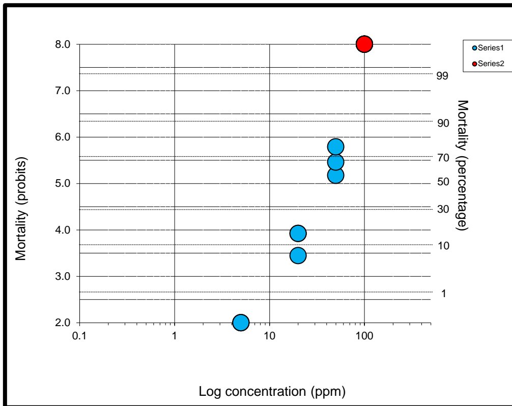
Figure 28. Response of Nasonovia ribisnigri clone to screening dose of pirimicarb applied at 100 ppm (red circles) super-imposed on the susceptible baseline response for this species (blue circles).
