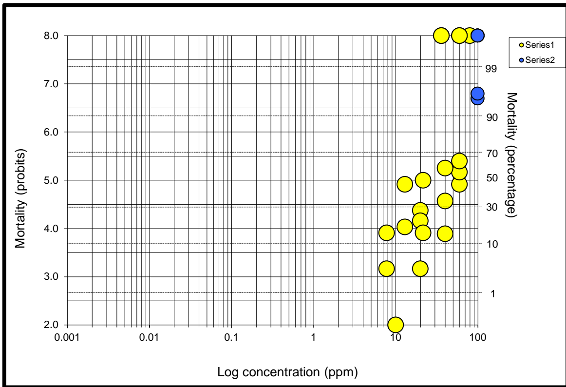
Figure 24. Response of Macrosiphum euphorbiae samples to screening dose of pirimicarb applied at 100 ppm (blue circles) super-imposed on the susceptible baseline response for this species (yellow circles).
