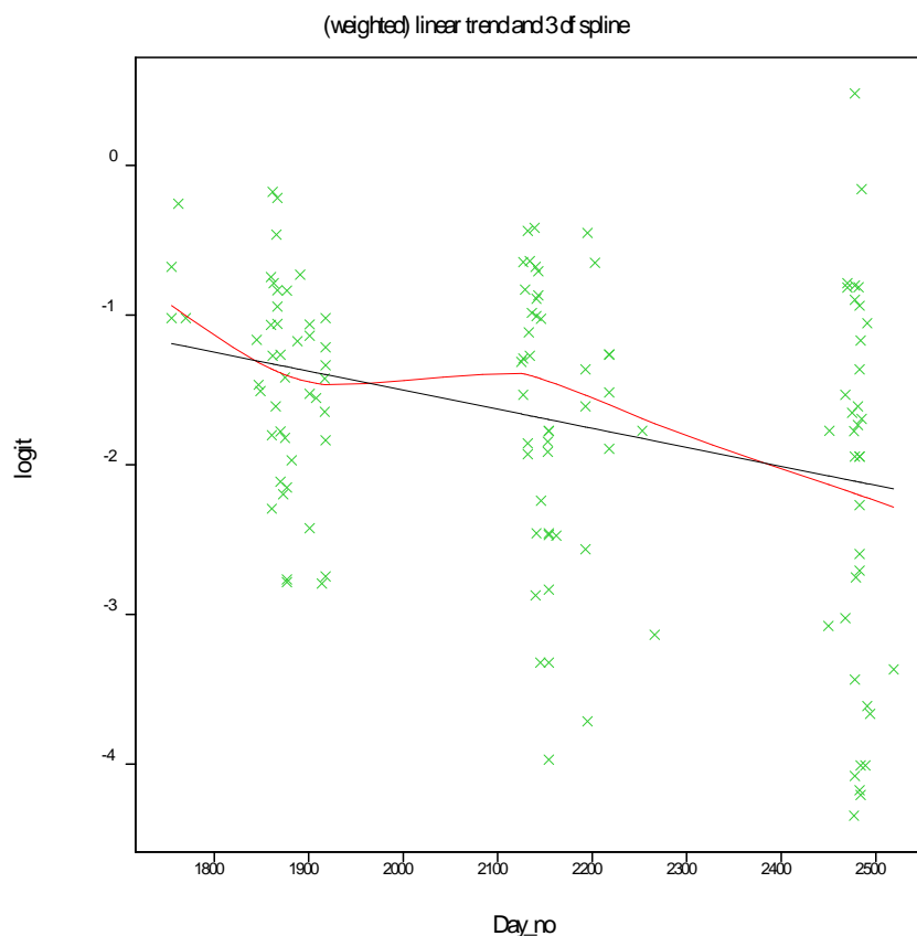
Figure 7. 3 df spline (red) fitted to logit transformed proportion of mobile nymphs in each field sample (after treatment with flonicamid) versus day number of collection. Black line shows linear component.
